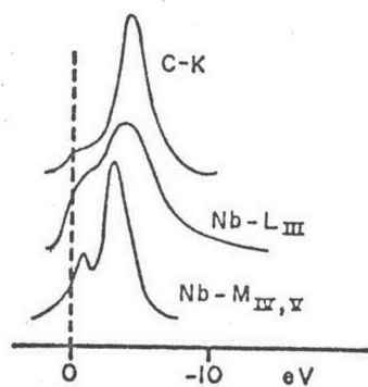
FIG. 9. NbC soft x-ray emission.
