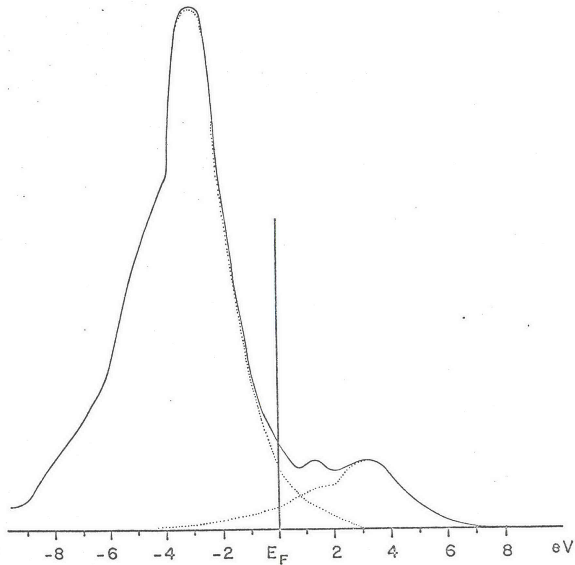
FIG. 10. TiC Ti-L II,III decomposition.
